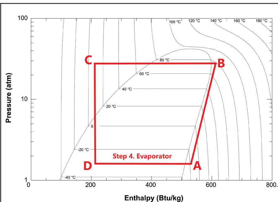
Figure 2: Mollier Diagram for R290 (propane). A vapor compression cycle (VCC) typically involves cycling the pressure, enthalpy and temperature through four stages: (Step 1) a compressor (A-to-B), (Step 2) a condenser (B-to-C), (Step 3) an expansion valve (C-to-D) and (Step 4) an evaporator (D-to-A). Step 3 happens when liquid propane expands and cools to subzero temperatures. Step 4 happens when energy is absorbed from the outdoor ambient as the liquid propane evaporates at constant pressure. This diagram was generated by REFPROP software. NIST Reference Fluid Thermodynamic and Transport Properties Database (REFPROP): Version 10. https://www.nist.gov/srd/refprop
